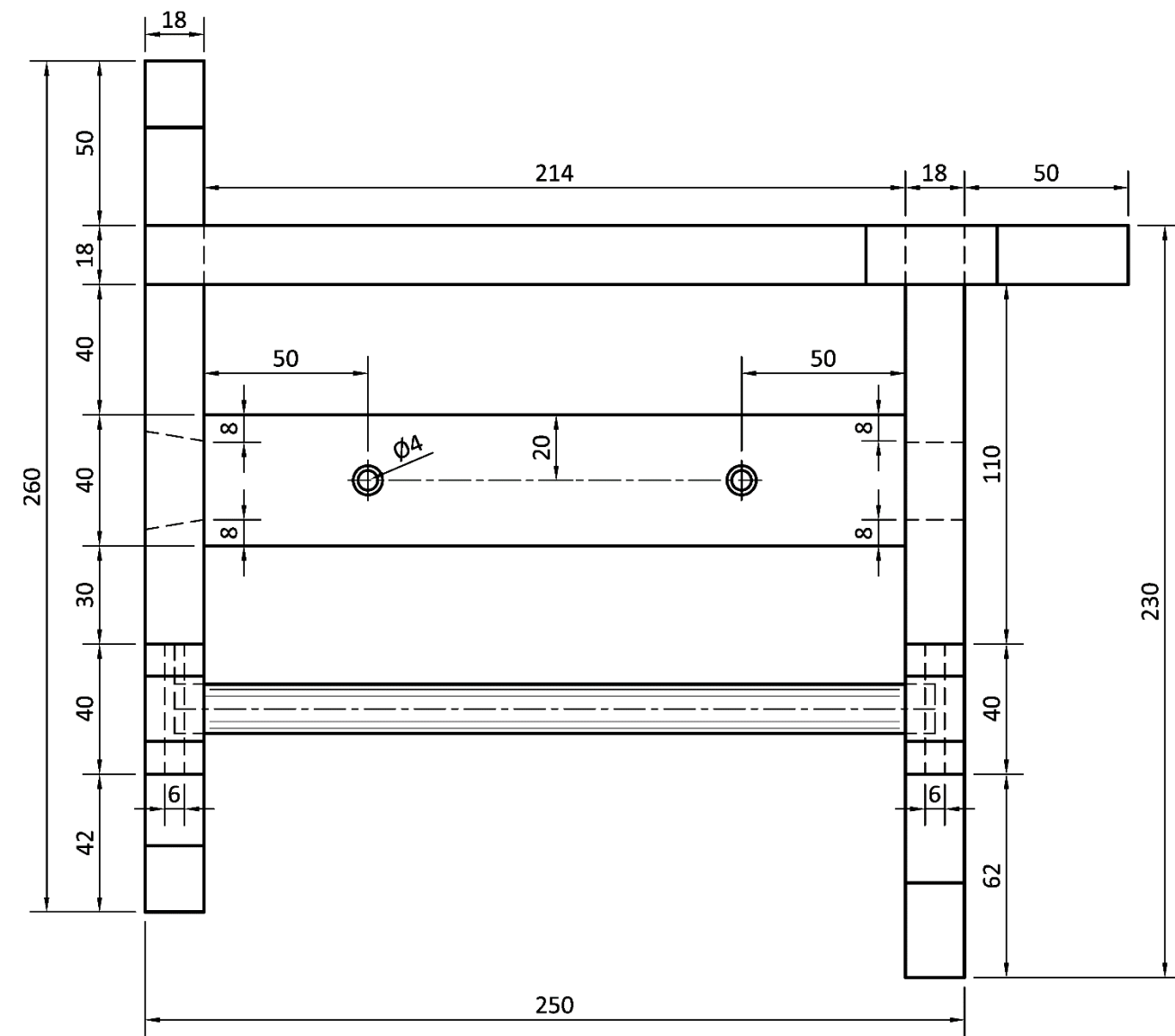
Elevation/Aghaidhchló
